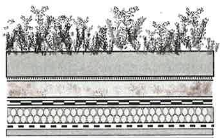
Built-in-place extensive green roof
